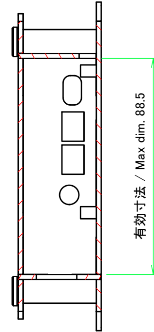
B-B (1:1.5)
